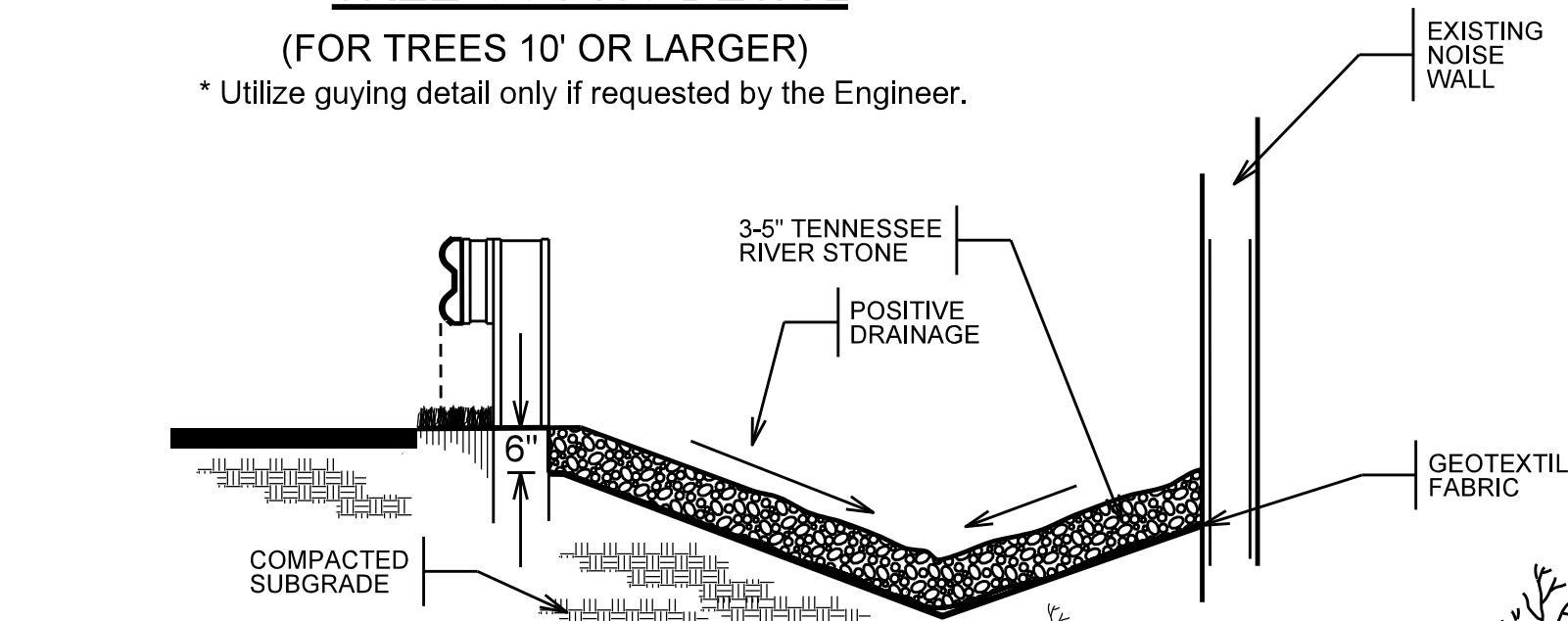
River Stone Detail No Scale
