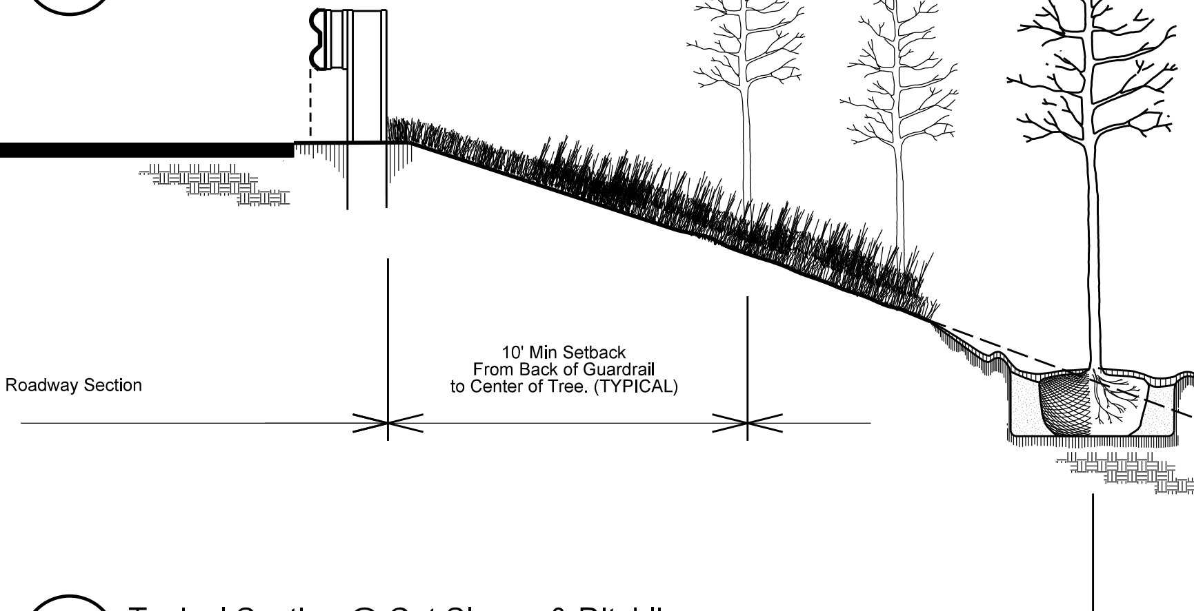
Typical Section @ Cut Slopes & Ditchlines No Scale
